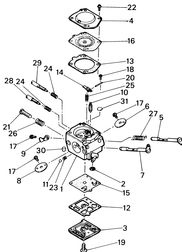
Fig.3 CARBURETOR COMPONENTS
