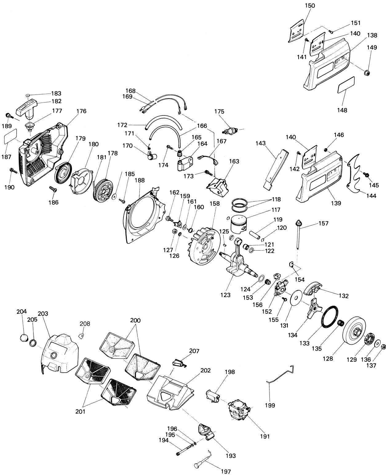
Fig.2 POWER UNIT
