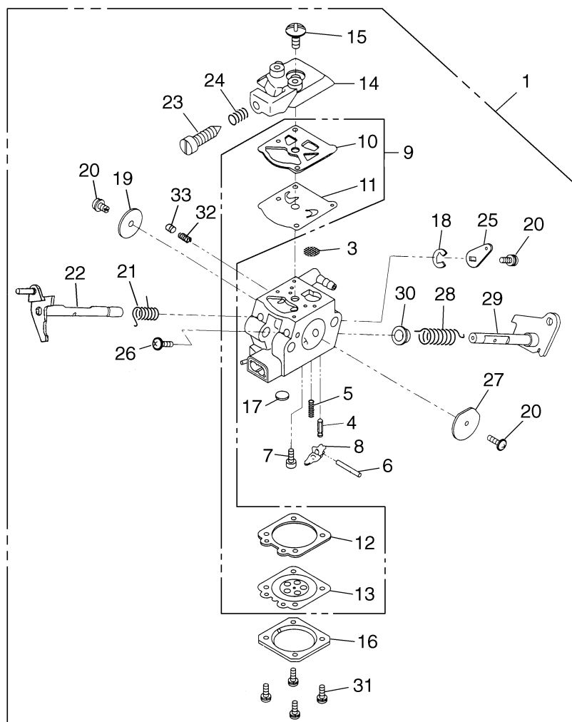
Fig.3 CARBURETOR COMPONENTS
