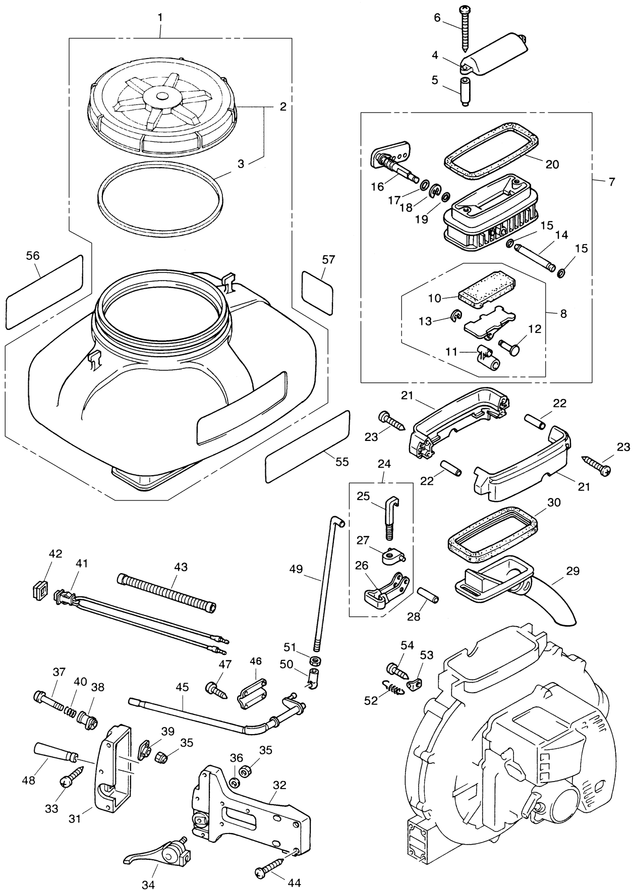
Fig.4 SPRAY GROUP (S/N 200101 and up)
