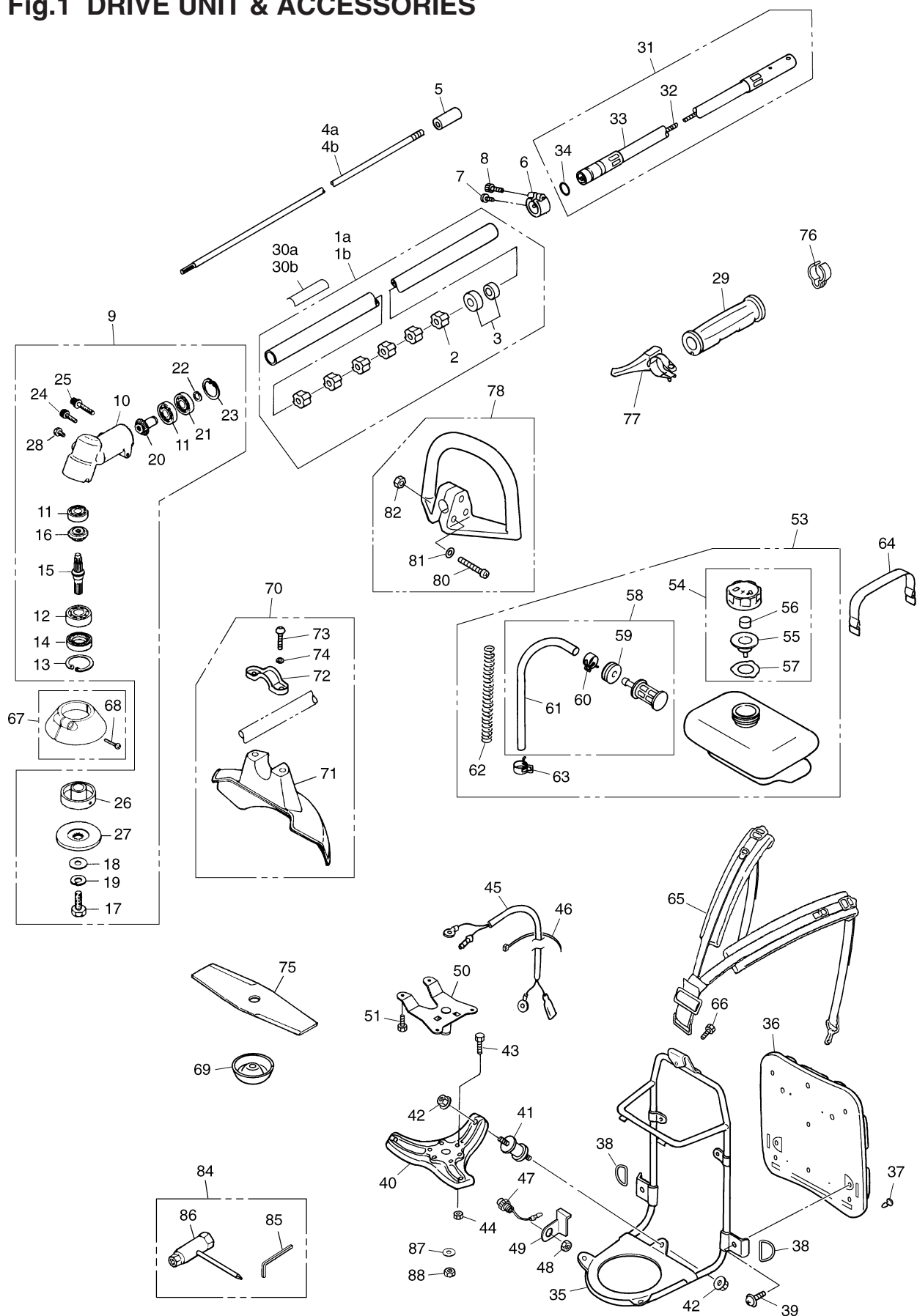
Fig.1 DRIVE UNIT & ACCESSORIES
