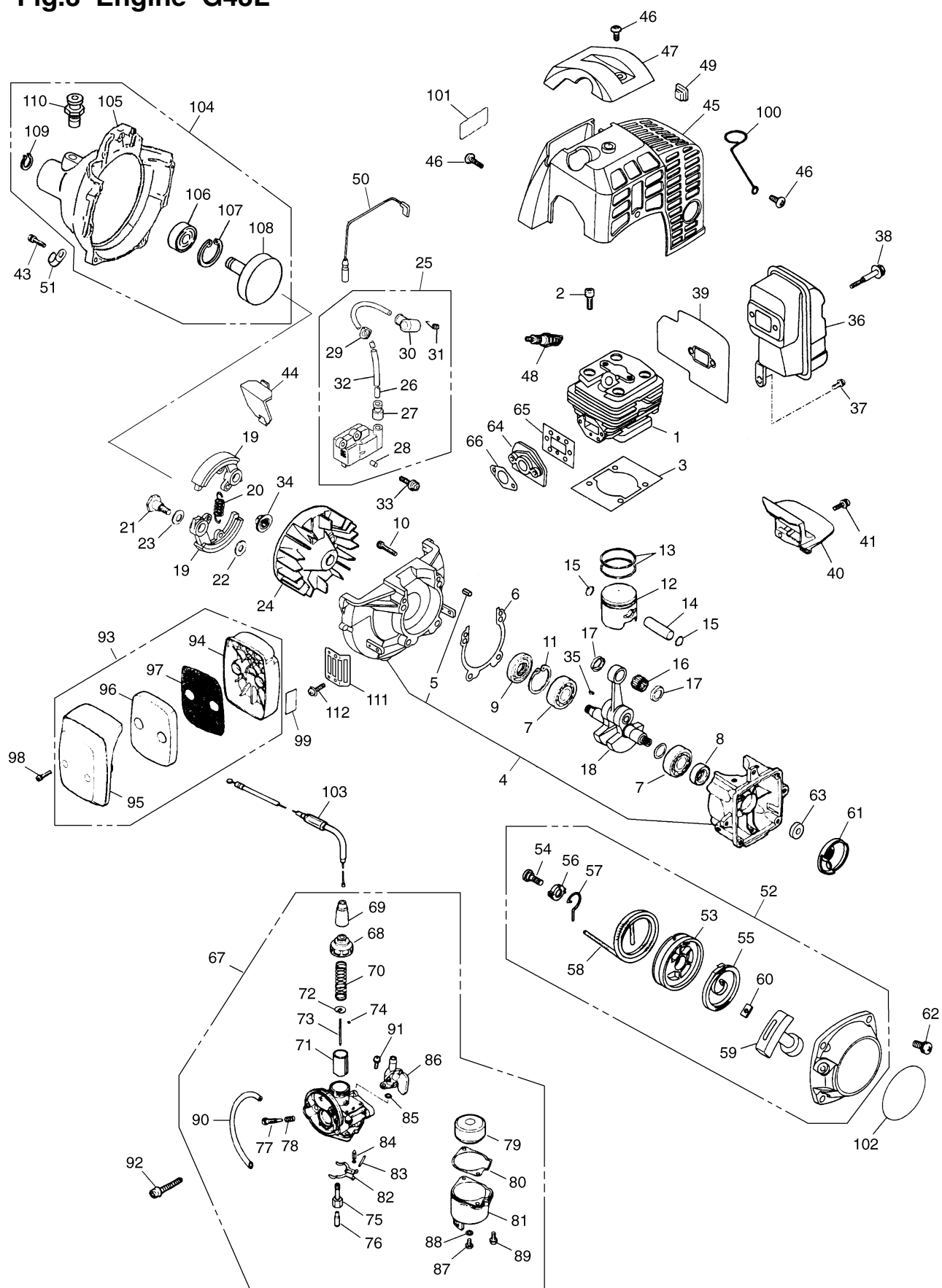
Fig.3 Engine G43L
