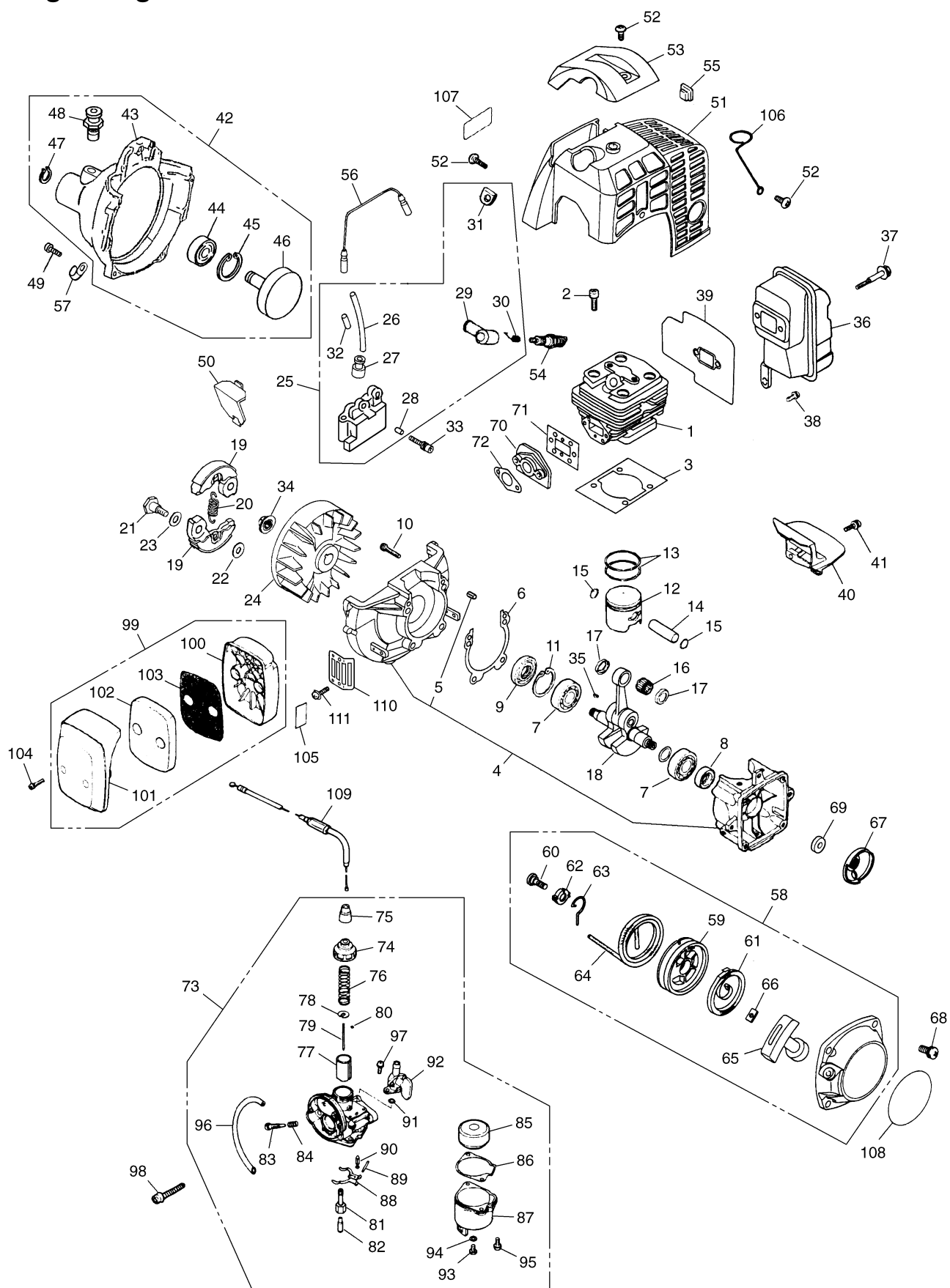
Fig.2 Engine G34L
