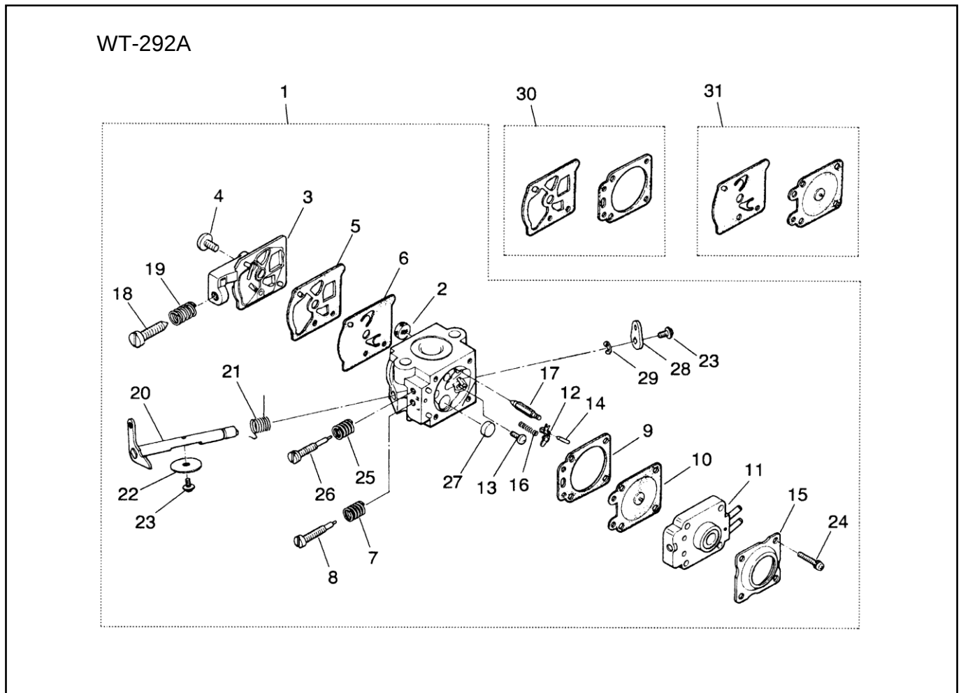
Fig.2 CARBURETOR COMPONENTS
