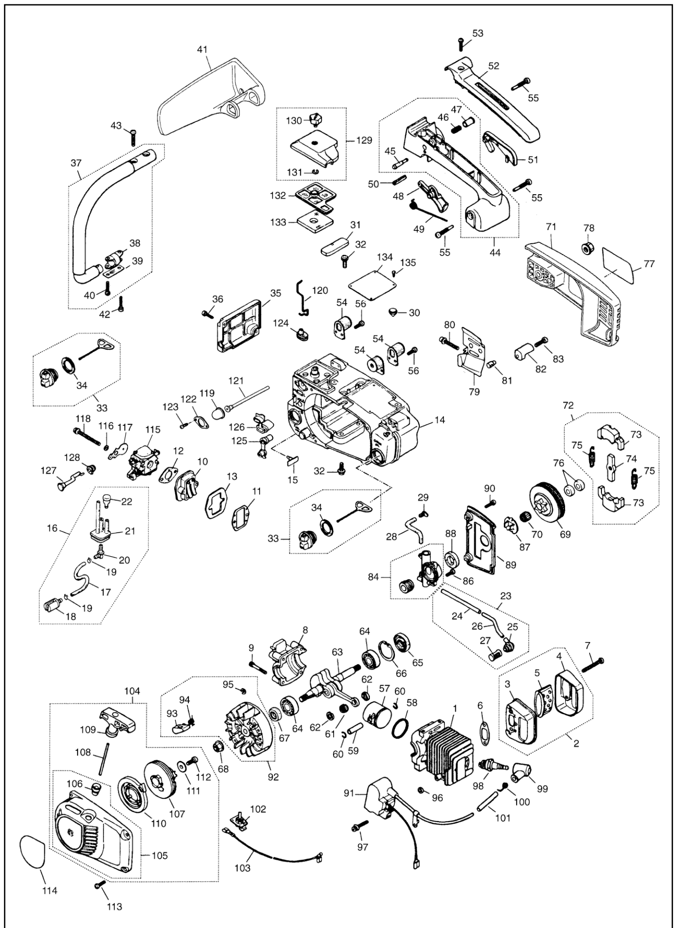
Fig.1 POWER UNIT
