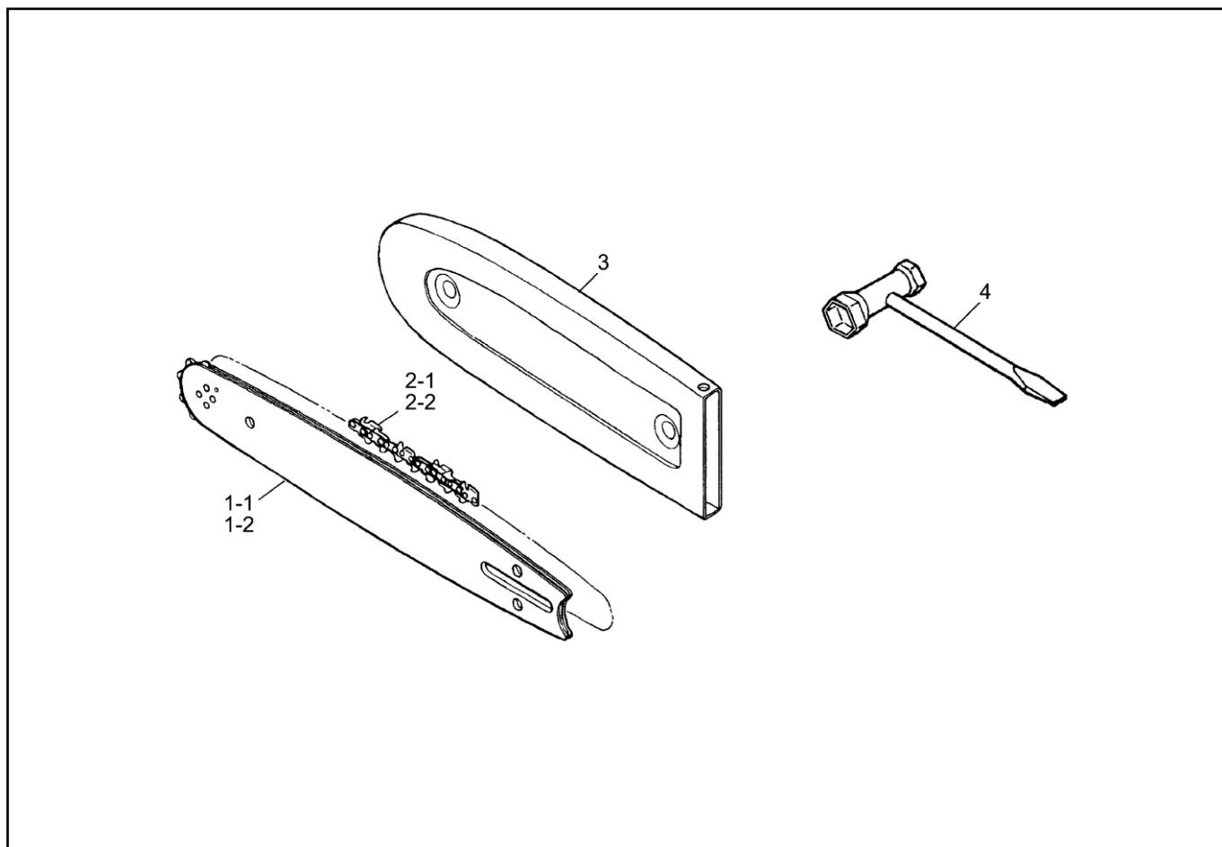
Fig.3 ACCESSORIES
